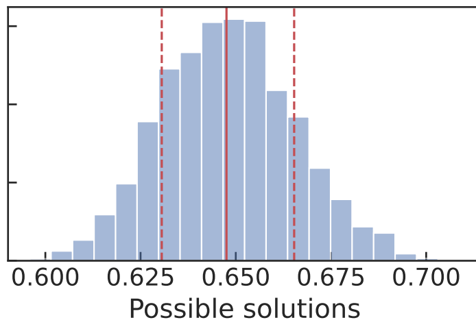
Radius of the star (in units of Solar radii) 0.648 \pm 0.018
