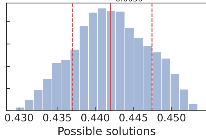
Mid-transit time (in units of days) 0.4420^{+0.0055}_{-0.0050}
