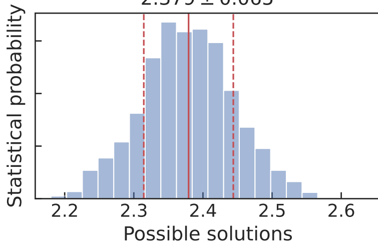
Radius of the planet (in units of Earth radii) 2.379 \pm 0.065
