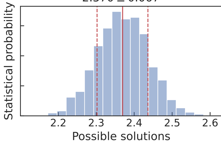
Radius of the planet (in units of Earth radii) 2.370 \pm 0.067
