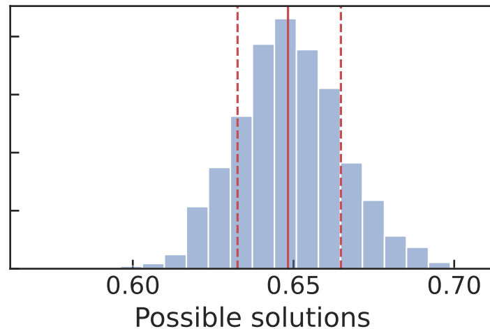
Radius of the star (in units of Solar radii) 0.648 \pm 0.016
