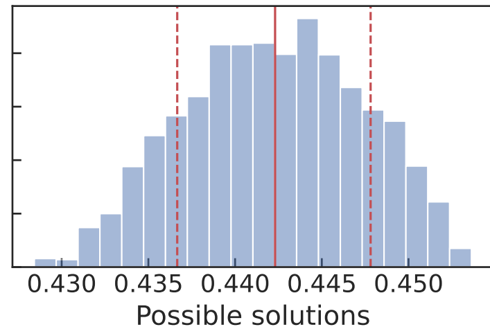
Mid-transit time (in units of days) 0.4423 \pm 0.0056
